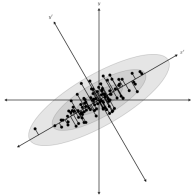
Figure 2.3: A distribution of points drawn from a bivariate Gaussian and centred on the origin of x and y . PCA defines a rotation such that the new axes ( x' and y' ) are aligned along the directions of maximal variance (the principal components) with zero covariance. This is equivalent to minimizing the square of the perpendicular distances between the points and the principal components
