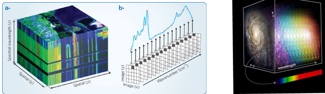
Figure 2.4: Illustrations of how a data cube looks like.
