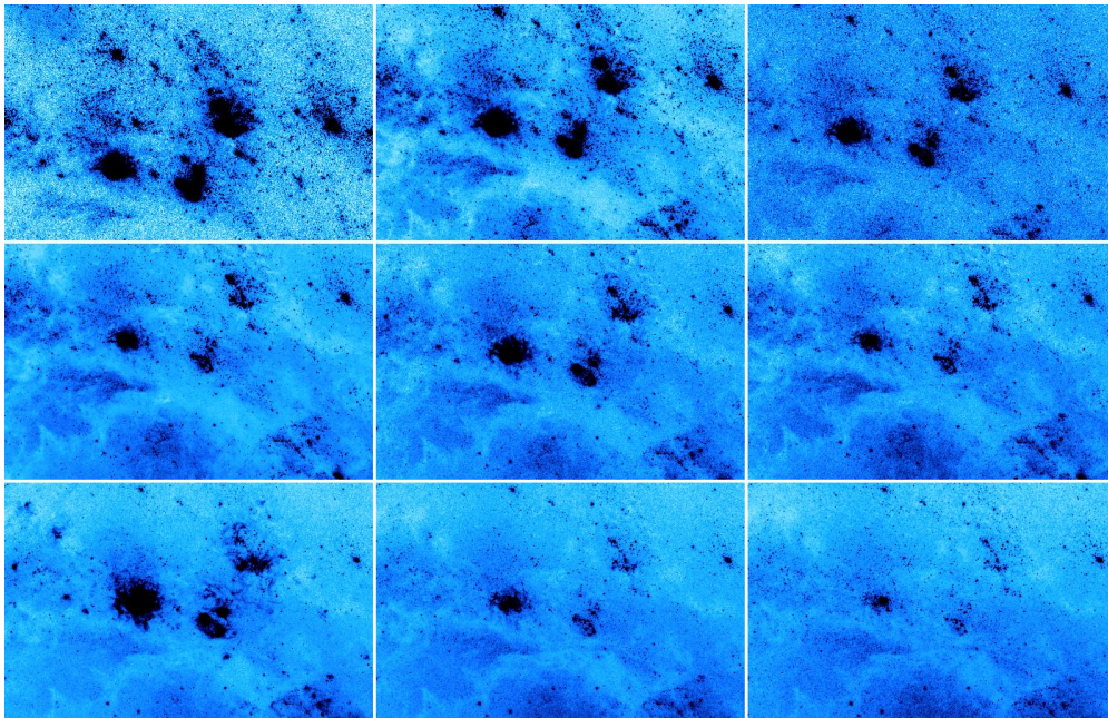
Figure 2.5: Example of how an object can look in 9 wavelengths
