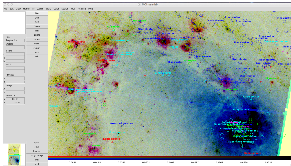
Figure 2.6: This is an RGB picture made from 3 independent FITS files, with a z scale and a region file overlaid from NED database, if you would like to learn more about this, or reproduce it, it is all explained in this web page: https://github.com/LaurethTeX/Clustering/blob/master/NEDtoREGION-FILE/KnownRegions.md
